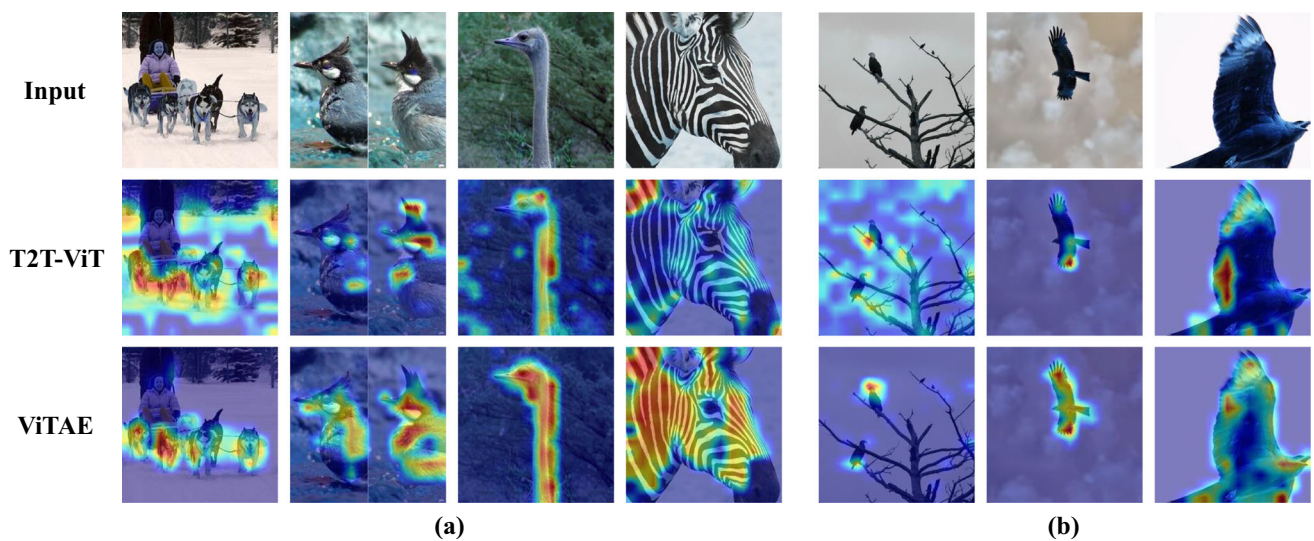
Fig. 4 Visual inspection of T2T-ViT-7 and ViTAE-T using Grad-CAM (Selvaraju et al., 2017). (a) Images containing multiple or single objects and the heatmaps obtained by T2T-ViT-7 and ViTAE-T. (b) Images con-
