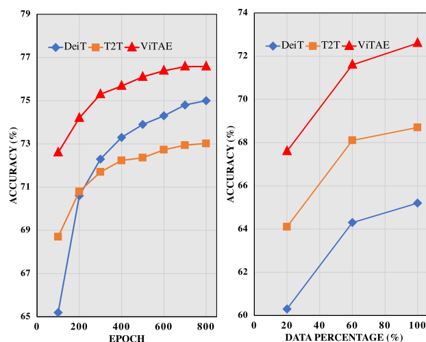
Fig. 1 Comparison of data and training efficiency of DeiT-T (Touvron et al., 2021a), T2T-ViT-7 (Yuan et al., 2021b) and ViTAE-T on ImageNet
